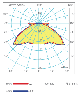
Light Distribution Curve
