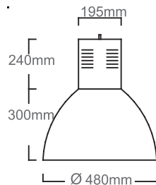
Technical Drawing
